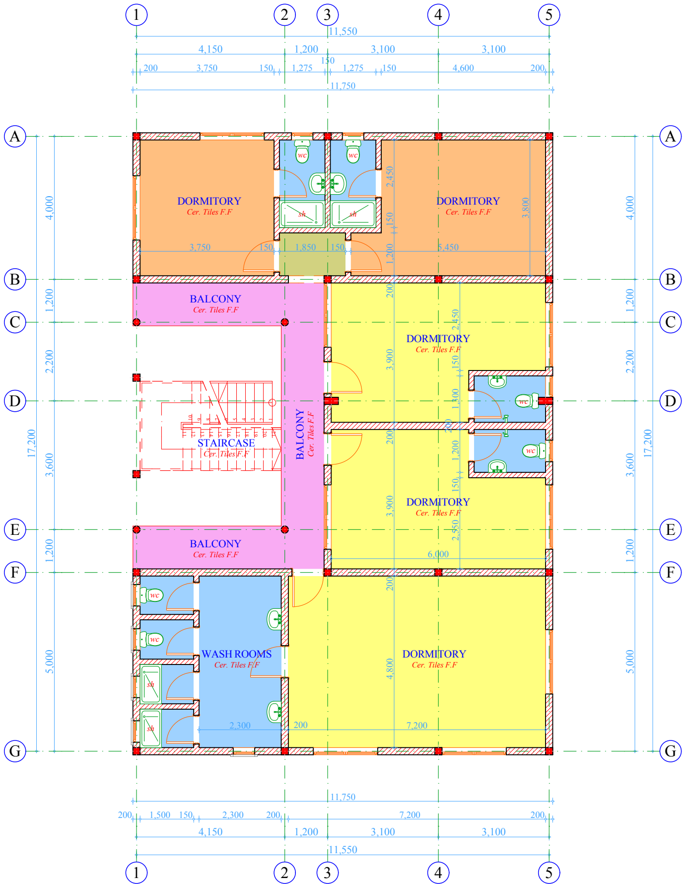
SECOND FLOOR PLAN Scale: 1:105
